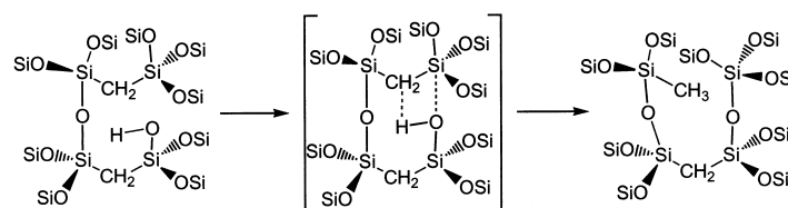
Scheme 2. Schematic representation of the cleavage of one Si-CH 2 bond to a bridging methylene group, leading to methyl groups terminally bonded to silicon.
